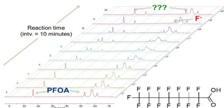
Characterization of PFOA Daughter Products
