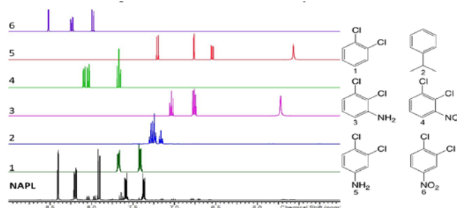
Non-Targeted Characterization of Complex NAPL Mixtures Using NMR Spectroscopy
