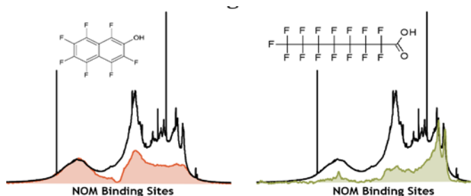
Contaminant Binding
